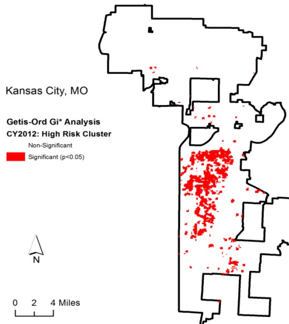
Figure 3. Getis-Ord G_i^* Analysis of High Risk Clusters for Kansas City, 2012
